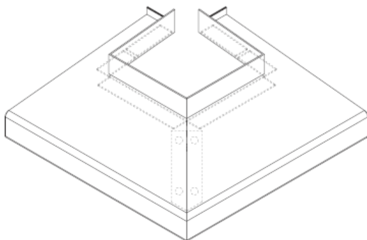
Angle AE - PB
